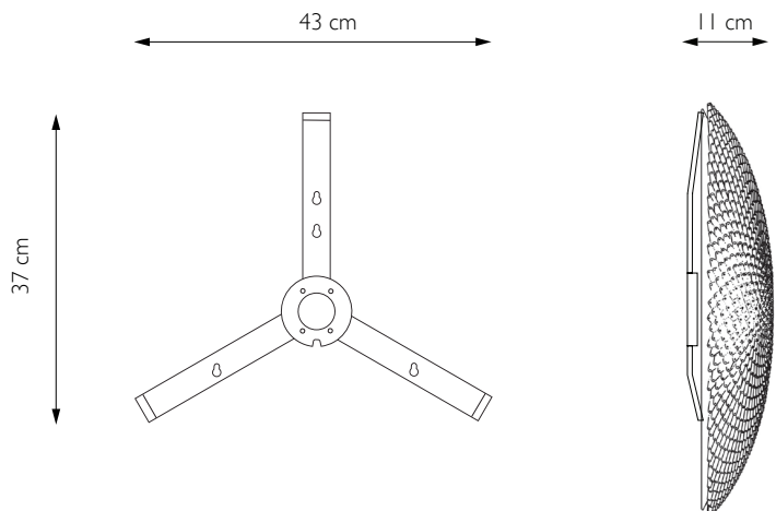
1597 ECO (shade Ø = 1597 D50)
